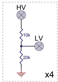
2/3 voltage divider
