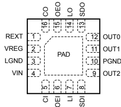
Pin-out Drawings
