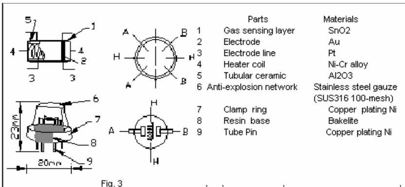
Structure and configuration of MQ-6 gas sensor is shown as Fig. 3, sensor composed by micro AL2O3 ceramic tube, Tin Dioxide (SnO2) sensitive layer, measuring electrode and heater are fixed into a crust made by plastic and stainless steel net. The heater provides necessary work conditions for work of sensitive components. The enveloped MQ-4 have 6 pin, 4 of them are used to fetch signals, and other 2 are used for providing heating current.
