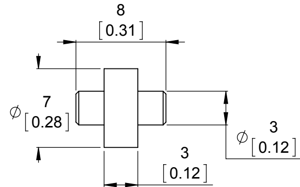
⑤ Ball bearing on dowel pin Scale 3:1
