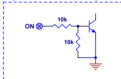
Input structure of ON input
