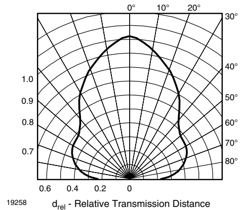
Fig. 9 - Horizontal Directivity
