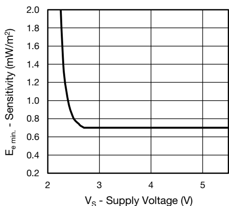
Fig. 11 - Sensitivity vs. Supply Voltage
