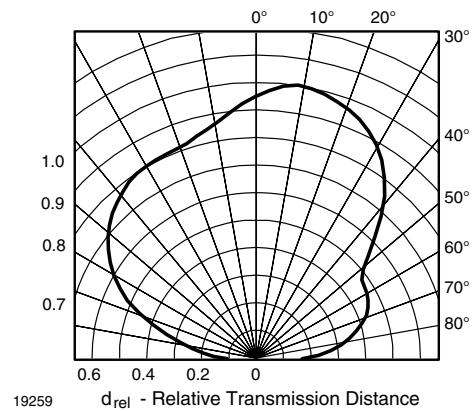
Fig. 10 - Vertical Directivity
