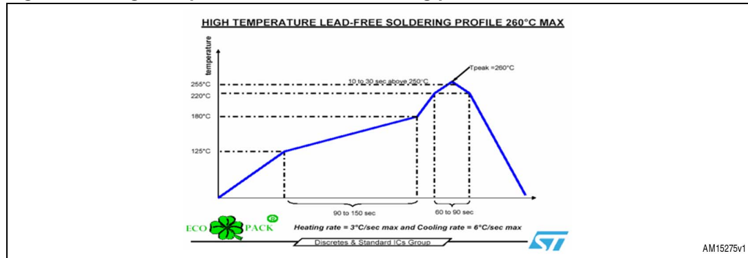
Figure 10. Example of solder machine profile
