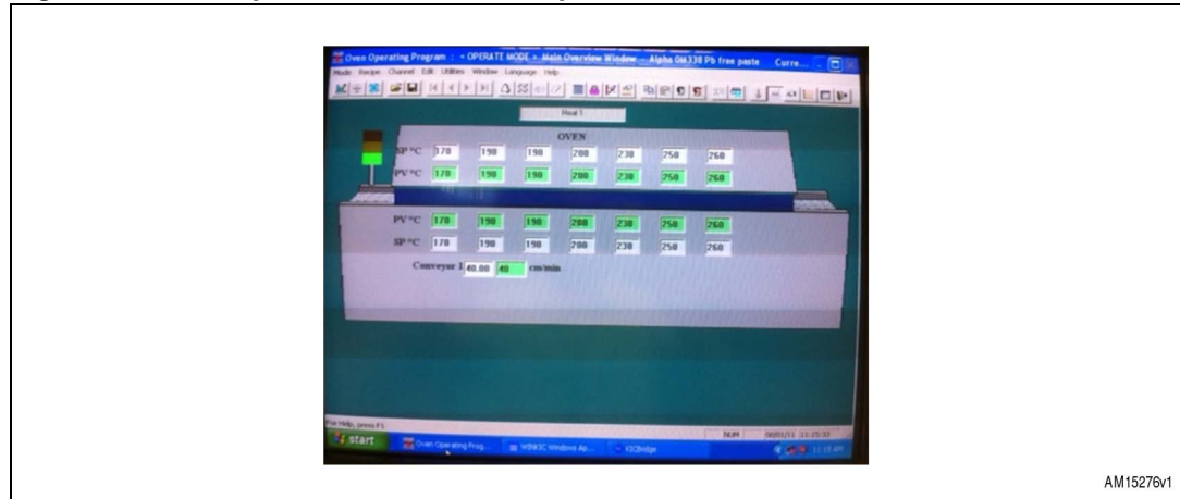
Figure 10. Example of solder machine profile
