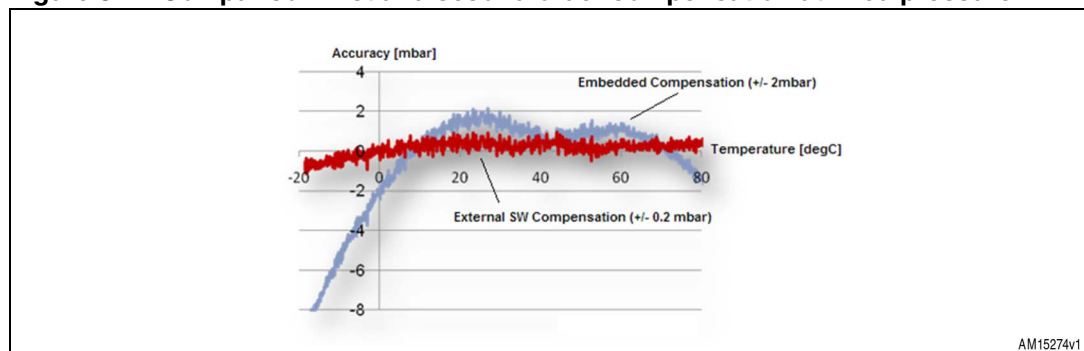
Figure 8. Comparison first and second order compensation at fixed pressure
