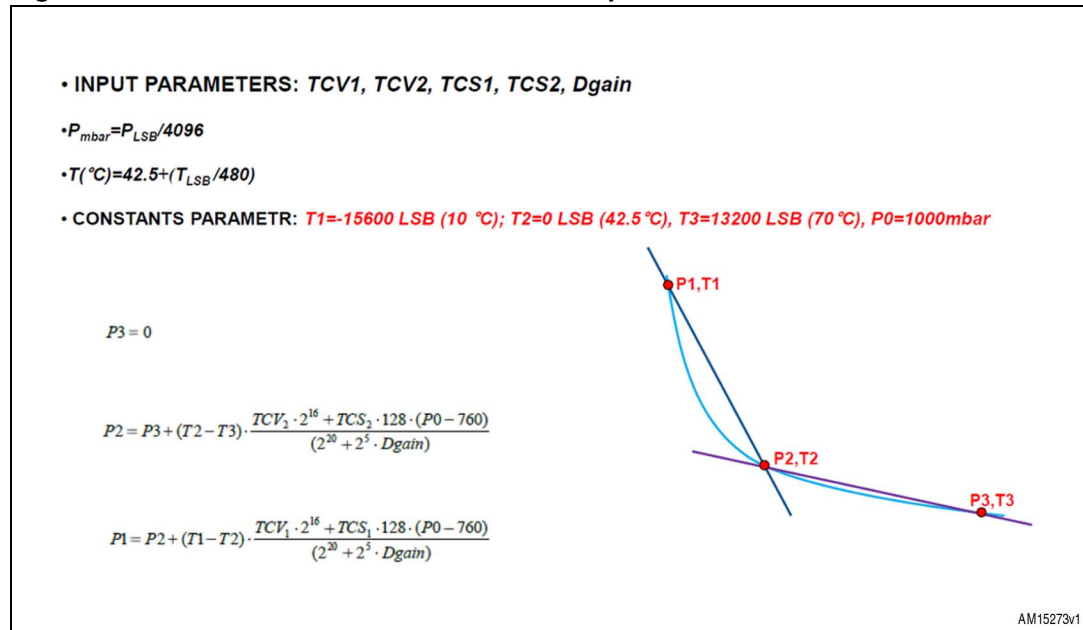
Figure 7. Overview first to second order compensation
