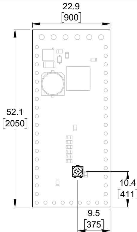
1 Board dimensions (top view) Scale 3:2
