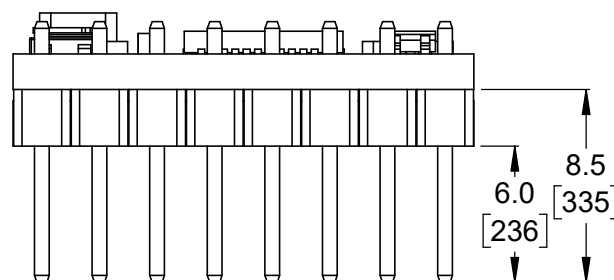
⑤ Profile with headers Scale 3:1
