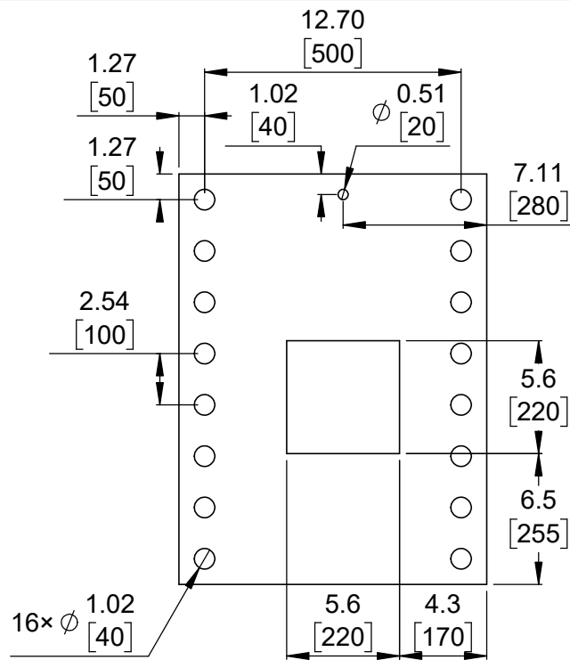
② Connector callouts (bottom view) Scale 3:1
