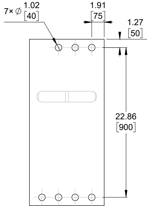
② Connector callouts (bottom view) Scale 3:1
