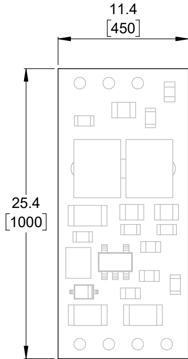
① Board dimensions (top view) Scale 3:1
