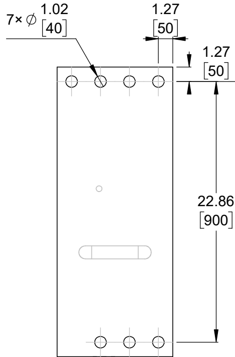
2 Connector callouts (bottom view) Scale 3:1
