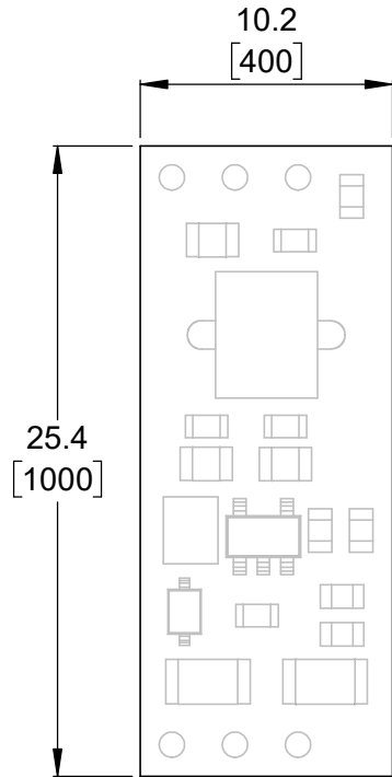
① Board dimensions (top view) Scale 3:1
