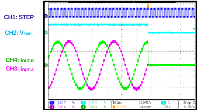
Output Disabled
