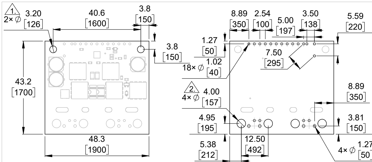
① Board dimensions (top view) Scale 1:1
