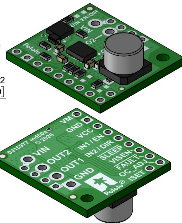
③ Isometric view Scale 5:2
