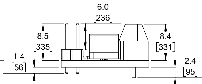
⑤ Profile (soldered connectors) Scale 5:2
