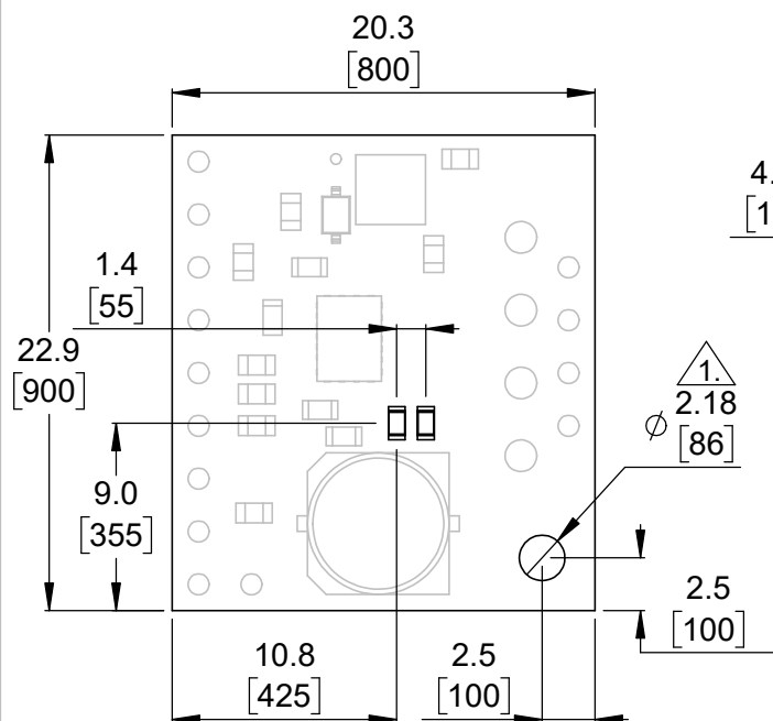
① Board dimensions (top view) Scale 5:2
