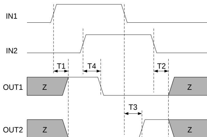
Figure 1: Input/Output Timing
