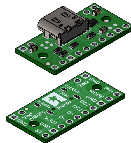
③ Isometric view Scale 2:1
