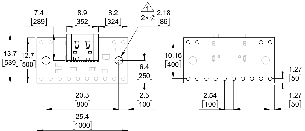
① Board dimensions (top view) Scale 2:1
