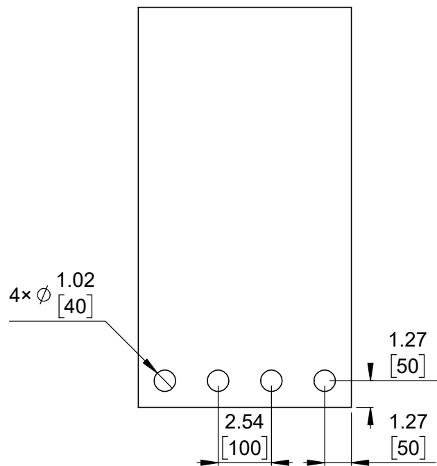
② Connector callouts (bottom view) Scale 4:1
