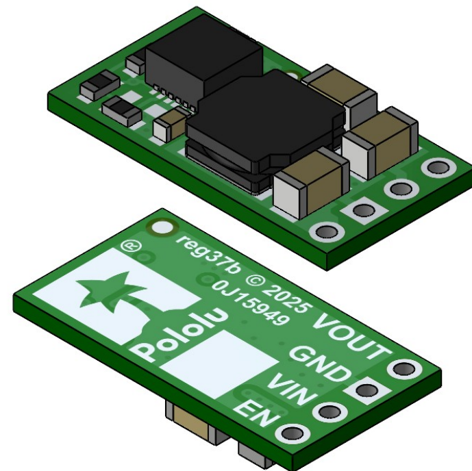
③ Isometric view Scale 4:1
