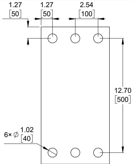
② Connector callouts (bottom view) Scale 5:1
