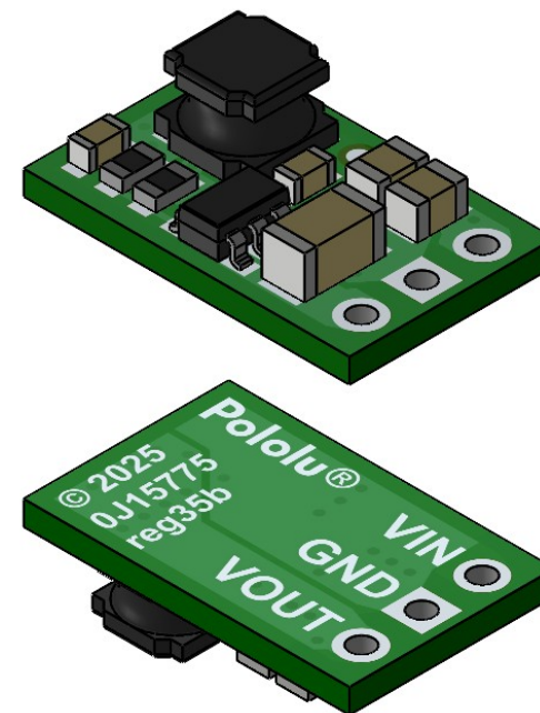
③ Isometric view Scale 4:1
