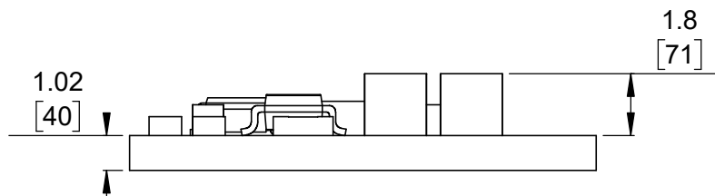
④ Profile Scale 5:1
