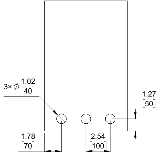
② Connector callouts (bottom view) Scale 5:1
