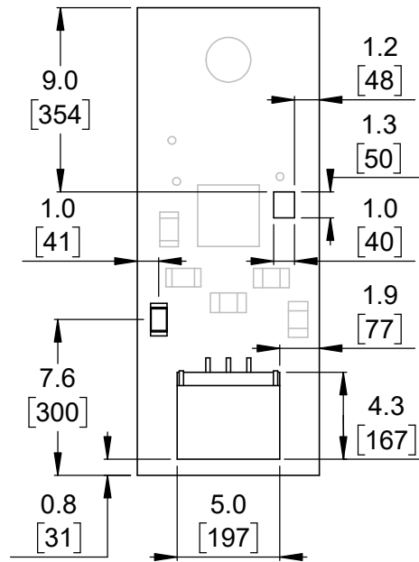
② User interface (bottom view) Scale 3:1
