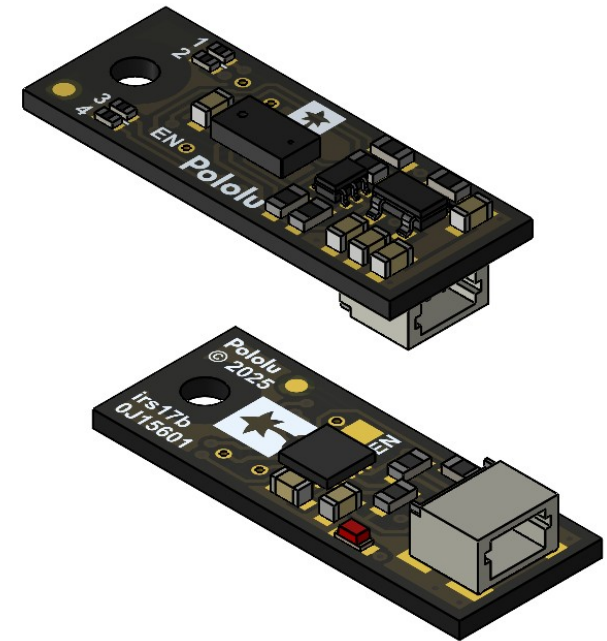
③ Isometric view Scale 3:1
