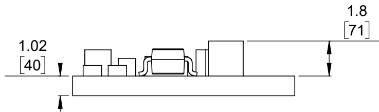
④ Profile Scale 5:1
