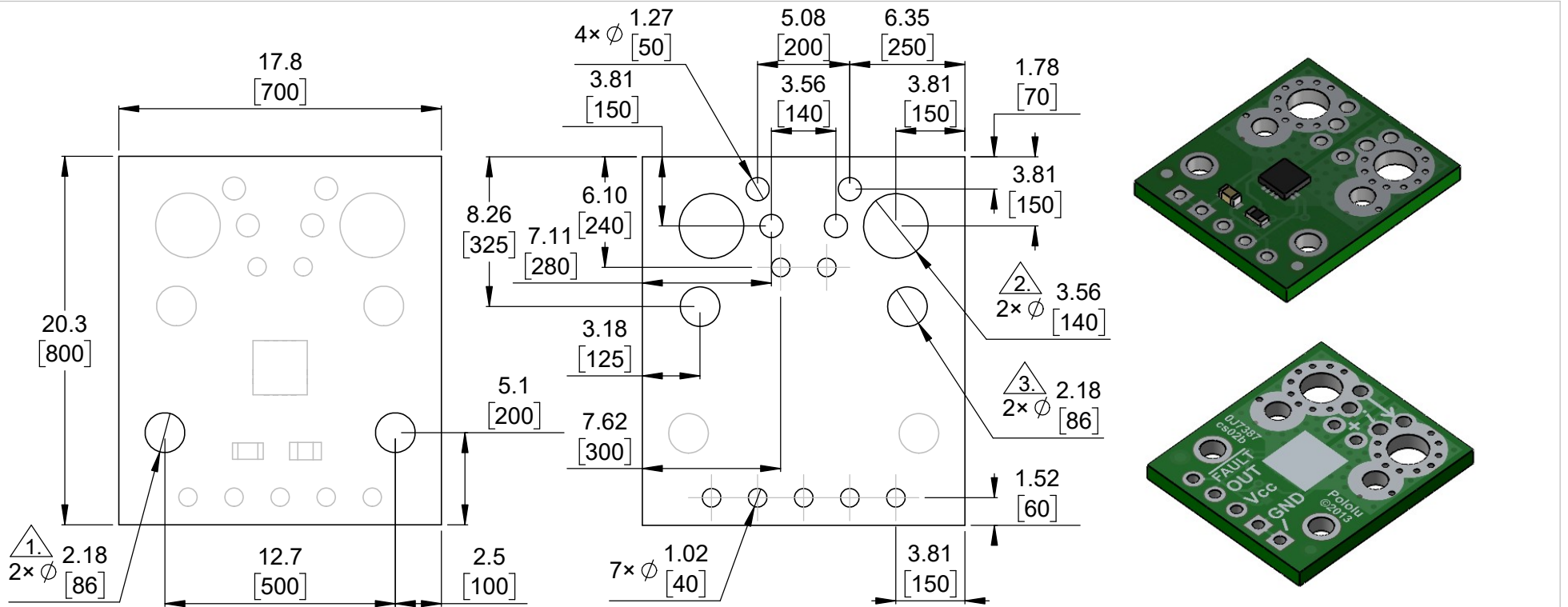
1 Board dimensions (top view) Scale 3:1
