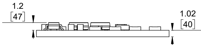
4 Profile Scale 3:1
