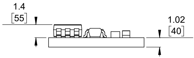
4 Profile Scale 4:1
