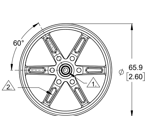
① Profile view without tire Scale 1:1
