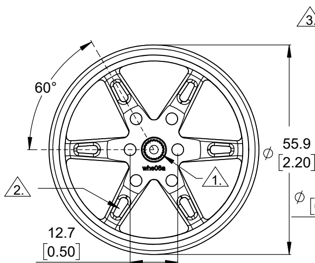
③ Back view without tire (actual size)
