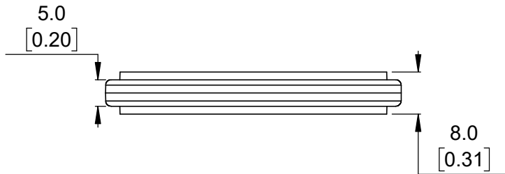
① Profile view without tire
