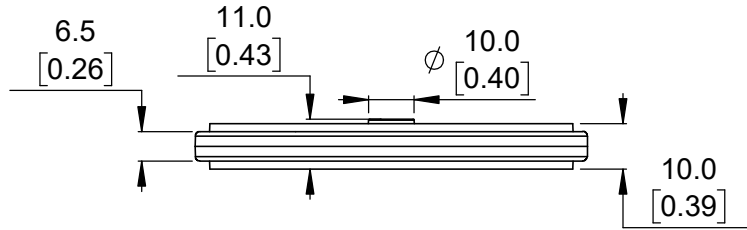
① Profile view without tire
