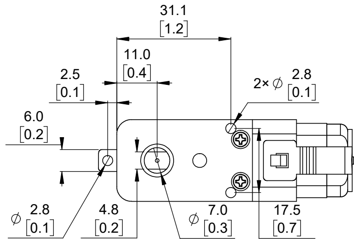
① Front view Scale 1:1
