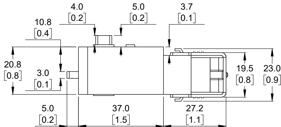
③ Top view Scale 1:1
