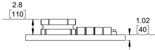
④ Profile Scale 3:1
