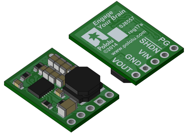
③ Isometric view Scale 3:1
