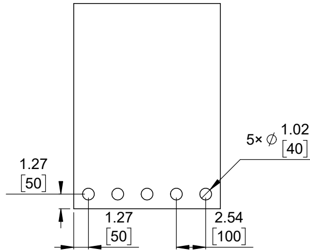
② Connector callouts (bottom view) Scale 3:1
