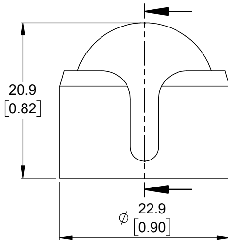
① Ball caster profile view Scale 2:1
