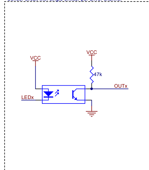
Sensor circuit with single emitter per driver channel**
