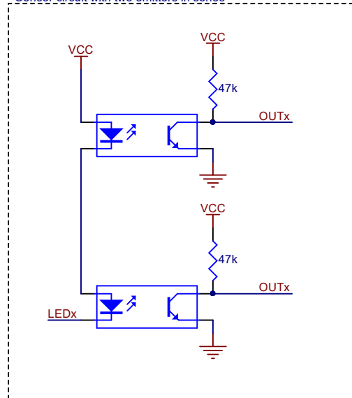
Sensor circuit with two emitters in series**
