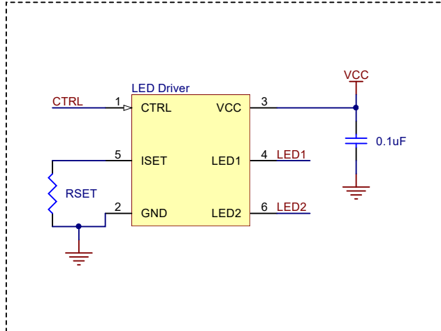
LED driver*
