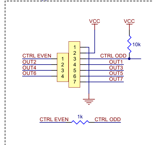
7 channel array pins
