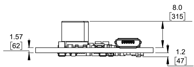
④ Profile Scale 3:2
