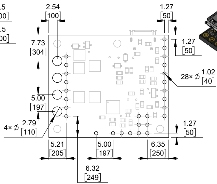
② Connector callouts (bottom view) Scale 3:2
