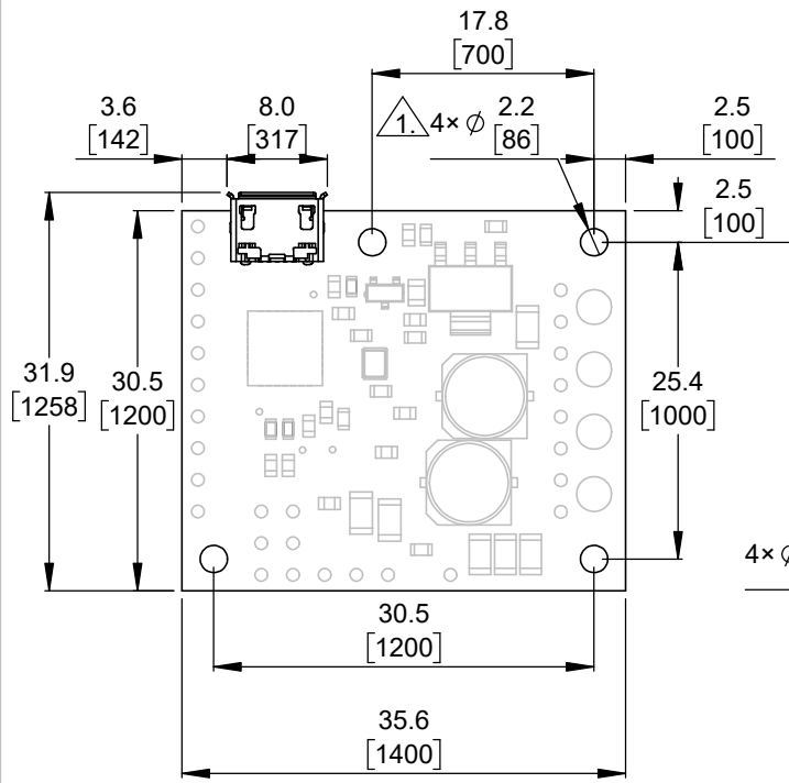
① Board dimensions (top view) Scale 3:2
