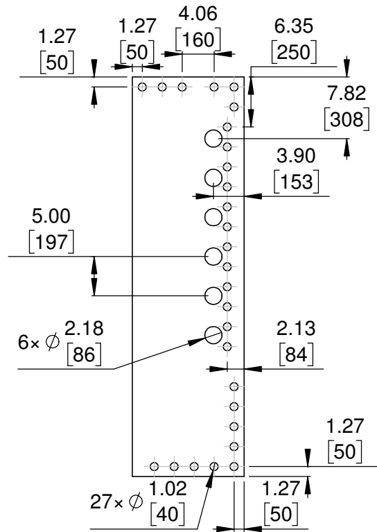
2 Connector callouts (bottom view) Scale 3:2
