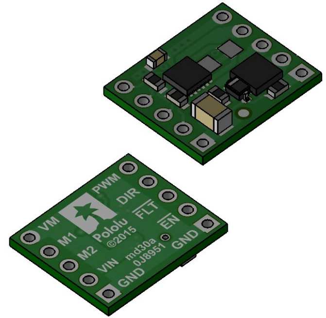
3 Isometric view Scale 3:1
