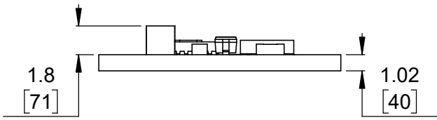
4 Profile Scale 3:1
