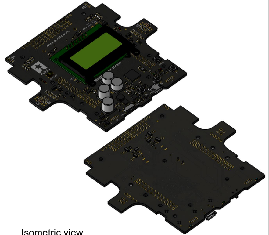
② Isometric view (with optional through-hole components and LCD) Scale 1:1
