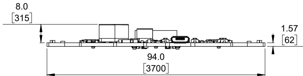
③ Long profile Scale 1:1
