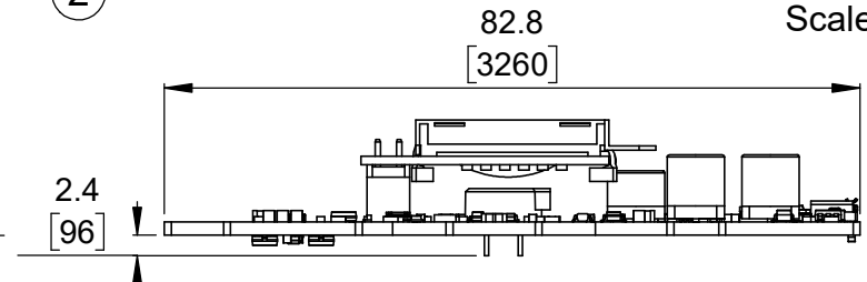
④ Short profile (with optional through-hole components and LCD) Scale 1:1
