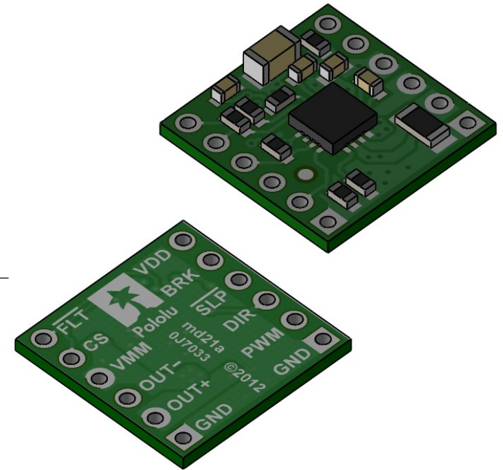
③ Isometric view Scale 3:1
