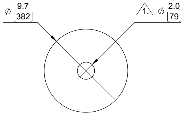
① Top view Scale 4:1
