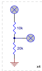
2/3 voltage divider
