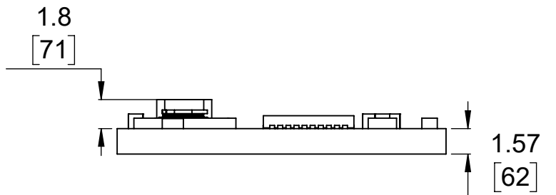
4 Profile Scale 3:1
