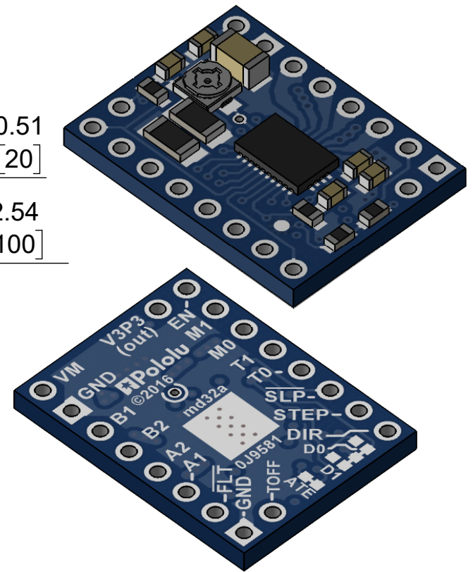
3 Isometric view Scale 3:1
