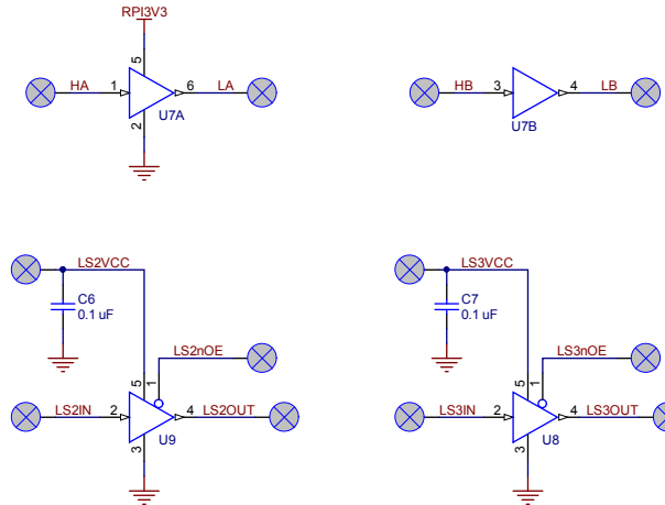
General-purpose dual unidirectional shifter
