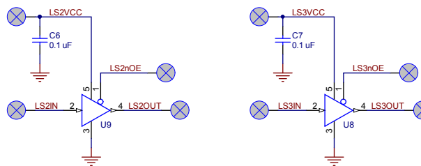
General-purpose tristatable unidirectional shifters
