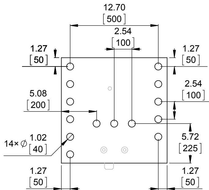
2 Connector callouts (bottom view) Scale 3:1
