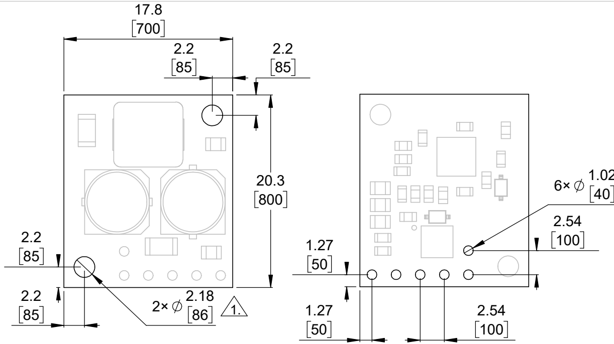
1 Board dimensions (top view) Scale 5:2
