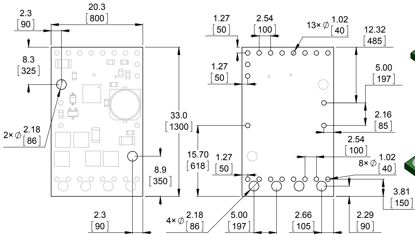
1 Board dimensions (top view) Scale 2:1
