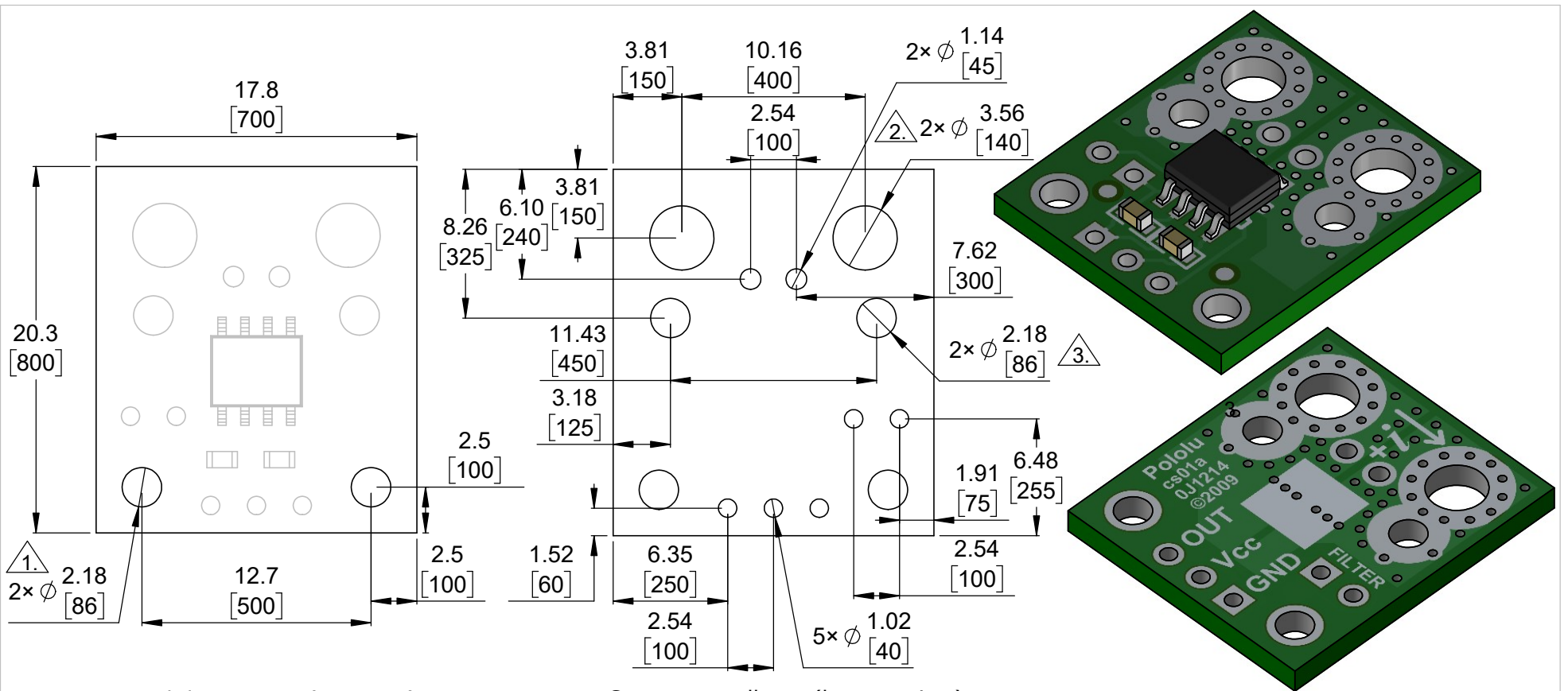
① Board dimensions (top view) Scale 3:1
