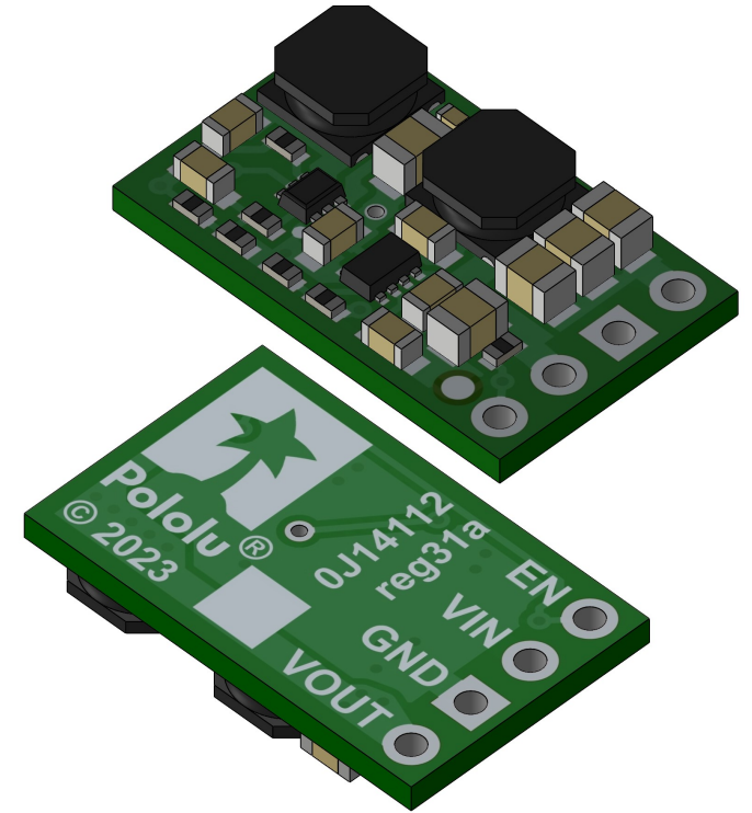
③ Isometric view Scale 4:1
