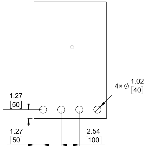
② Connector callouts (bottom view) Scale 4:1
